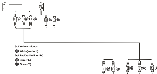
VIDEO EQUIPMENT with YPbPr
